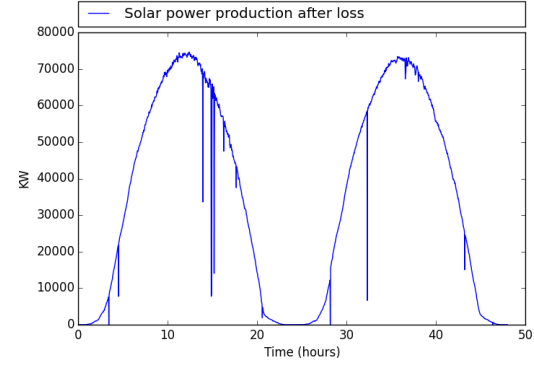
Fig. 4. Solar panel production for the experiments
