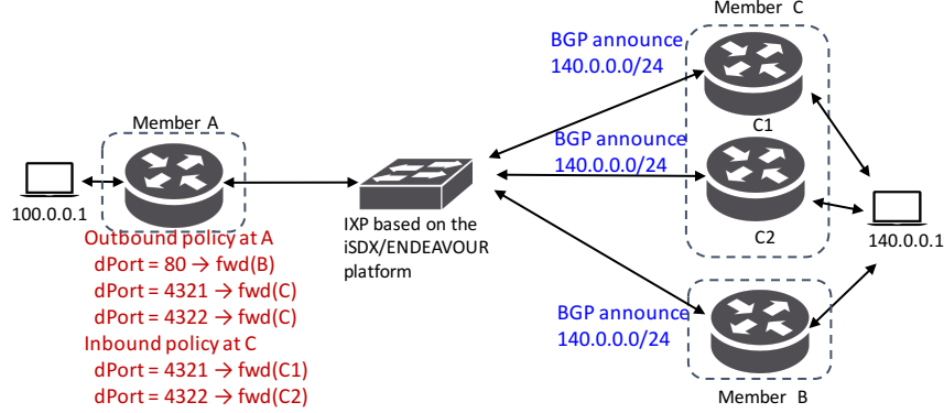
Figure 1: Simplified IXP based on the ENDEAVOUR platform for the In-bound/Outbound TE use case.
