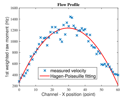
Fig. 3. 50 \mu\text{L}/\text{min} flow profile measured (with fitting curve)
