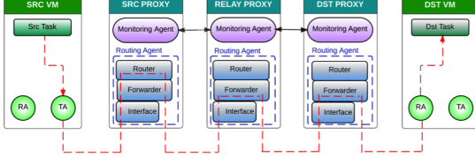
Fig. 4. Details of the SMART packet forwarding process.
