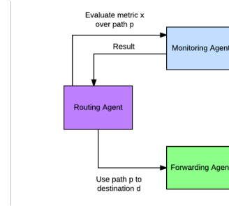
Fig. 3. Interactions between the entities constituting the proxy.
