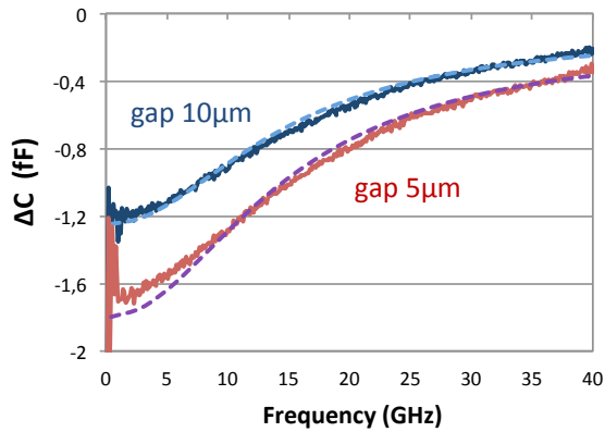
Fig. 2. Simulated and measured capacitive contrasts of polystyrene beads of 10 \mu\text{m} diameter for a capacitive sensor gap of 10 \mu\text{m} width.
