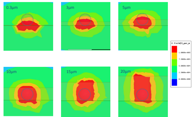
Fig. 7 EM field distribution in the sensor and bead for different CPW metal thicknesses (for a bead's diameter: 10 μm and a capacitive gap of 10 μm).
