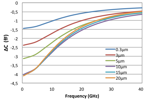
Fig. 3. Capacitive contrast of a polystyrene bead of 10 \mu\text{m} of diameter for gold waveguide thicknesses comprised between 0.3 \mu\text{m} and 20 \mu\text{m} .
