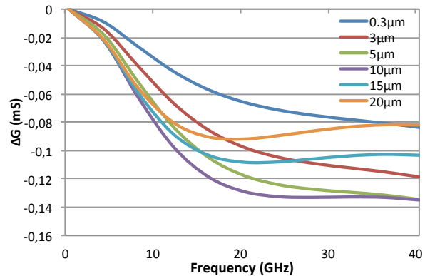
Fig. 4. Conductive contrast of a polystyrene bead of 10 \mu\text{m} of diameter for gold waveguide thicknesses comprised between 0.3 \mu\text{m} and 20 \mu\text{m} .
