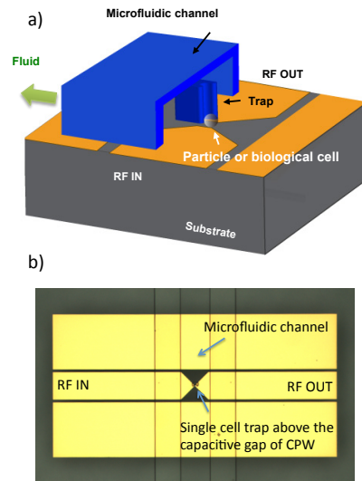
Fig. 1. a) Schematic and b) photograph of the microwave biosensor dedicated to the microwave spectroscopy of individual particle or biological cell.
