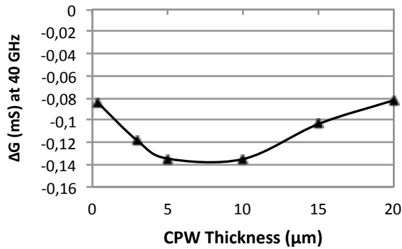
Fig. 6. Variation of the conductive contrast versus gold CPW thickness.
