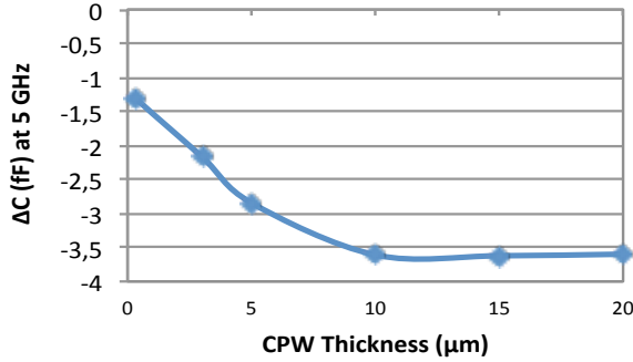
Fig. 5. Variation of the capacitive contrast versus gold CPW thickness.
