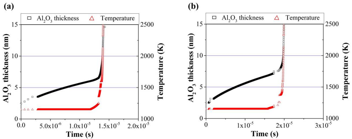
FIG. 13. Time dependence of the alumina thickness and temperature at the bottom of the thermite for a thermite composed of 8 bilayers of thickness 150 nm (a) deposited on heater 1 (heating surface area of 1.04 \times 10^{-2} \text{ cm}^2 ). (b) deposited on heater 3 (heating surface area of 2.51 \times 10^{-3} \text{ cm}^2 ).
