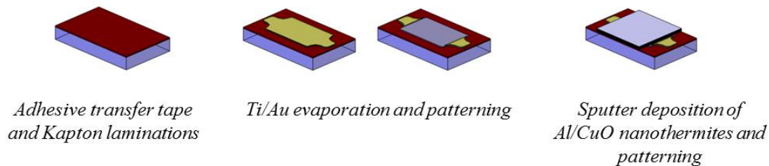
FIG. 1. 3D schematic views of main process steps.
