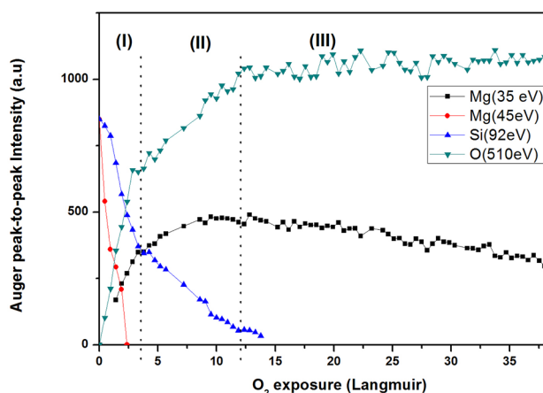
FIG. 5. Auger peak-to-peak signals of Mg, Si, and O as a function of \text{O}_2 exposures during in-situ oxidation process at RT ( P_{\text{O}_2} = 1 \times 10^{-8} T) of one Mg monolayer.
