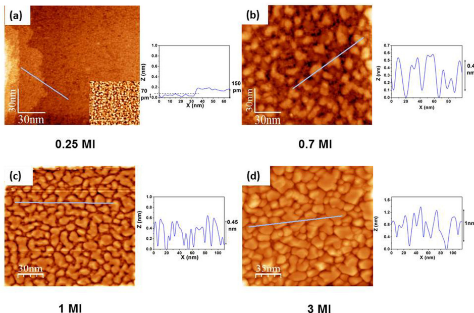
FIG. 3. Topographic STM images of the Mg deposit onto Si(100)-2 × 1 recorded for different coverages and corresponding height profiles. (a) 150 × 150 nm 2 empty state STM image after 0.25 ML of Mg deposition. (b) 150 × 150 nm 2 empty state STM image after 0.7 ML. (c) 150 × 150 nm 2 filled state STM image for 1 ML deposited. (d) 175 × 175 nm 2 filled state STM image after 3 deposited ML.
