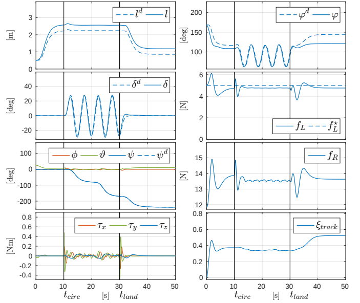
Fig. 4. Simulation results with parameters uncertainties (case b).
