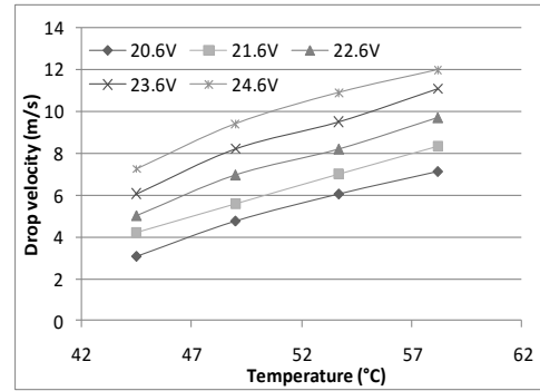
FIG.5. Temperature effect on the velocity of DC704 silicon oil at different pulse amplitude.
