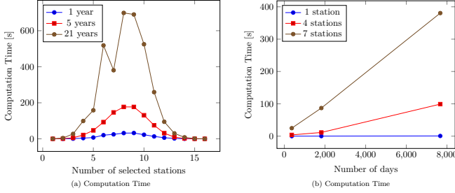
Fig. 1: Computation time for \mathcal{N}_{16}
