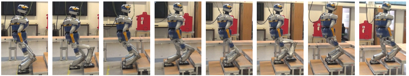
(a) Snapshots of the climbing up 10-cm high steps motion with the HRP-2 robot.
