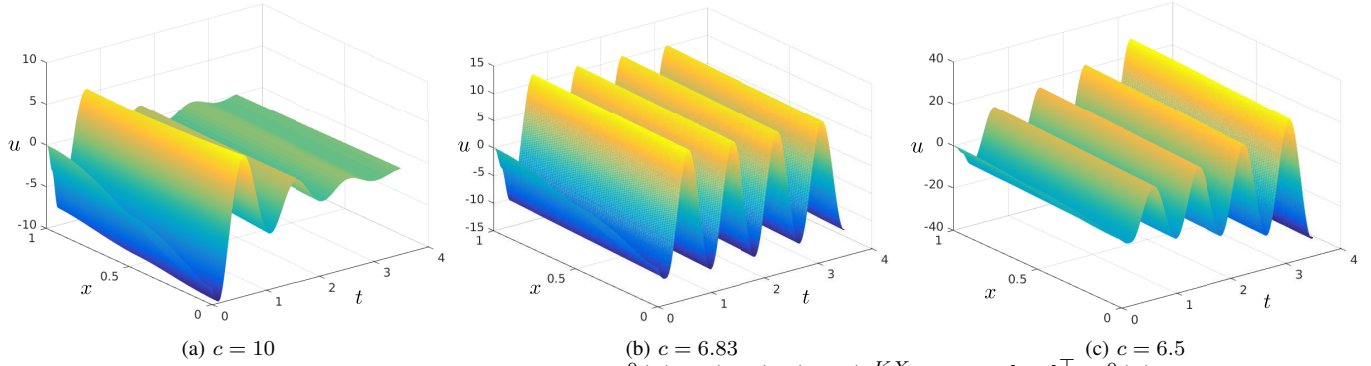
Fig. 2: Chart of u for system (29) with the parameters: u^0(x) = (\cos(\pi x) + 1) \frac{KX_0}{2} , X_0 = [1 \ 1]^\top , v^0(x) = 0 and c_0 = 0.15 for 3 values of c . These results are obtained using Euler forward as a numerical scheme.
