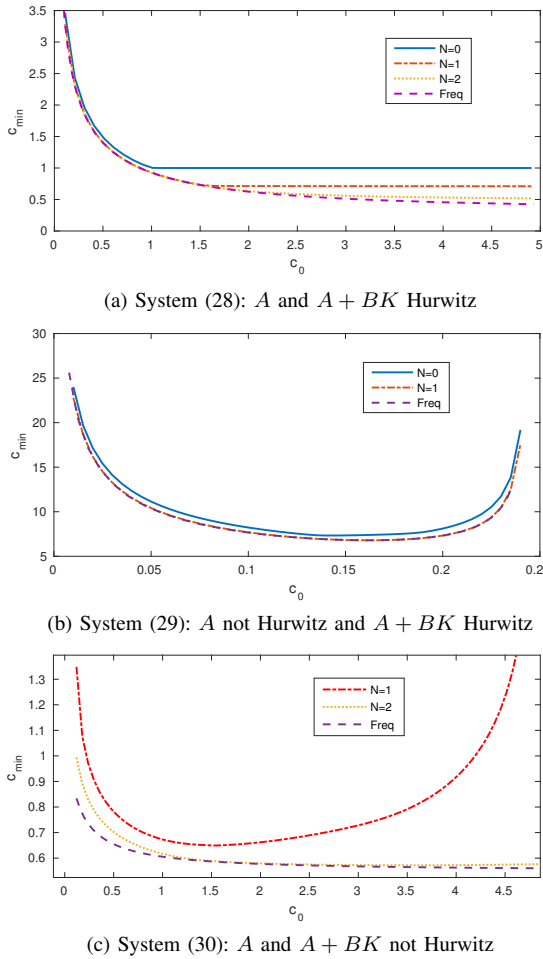
Fig. 1: Minimum wave speed c_{min} as a function of c_0 for system (1) to be stable. The values for A , B and K are given by equations (28), (29) or (30).
