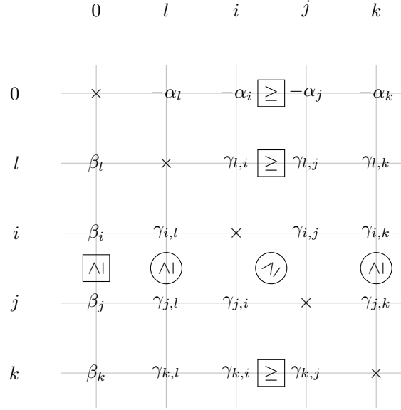
Figure 1: Illustration of Lemma 5: \bigcirc \geq imply \boxed{\geq} .
