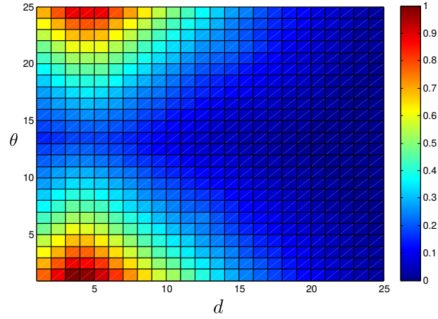
Fig. 7. Naive Global Planner learned state environment, red value is the maximum V Value for each state. The image displayed correspond to the 25x25 grid.
