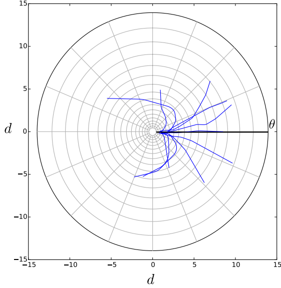
Fig. 5. Demonstration of the robot approaching the target person. Values of N = 16 and M = 16 for the state space. The darker black line represents the front of the person.
