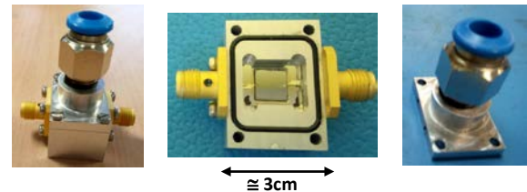
Figure 6: View of the packaged sensor
