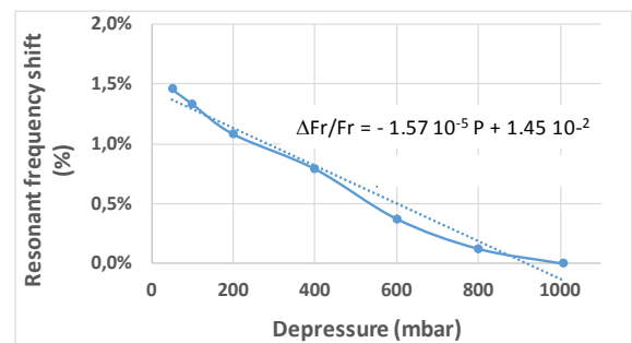
Figure 8: Measured resonant frequency shift versus depression
