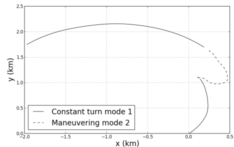
Fig. 3. Example of randomly generated trajectory for coordinated turn model
