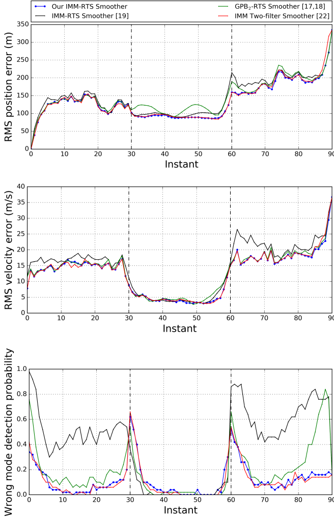
Fig. 2. Comparison of the IMM filter and the smoothers: (from top to bottom) (a) RMSE in Position, (b) RMSE in Velocity and (c) Mode error probability.
