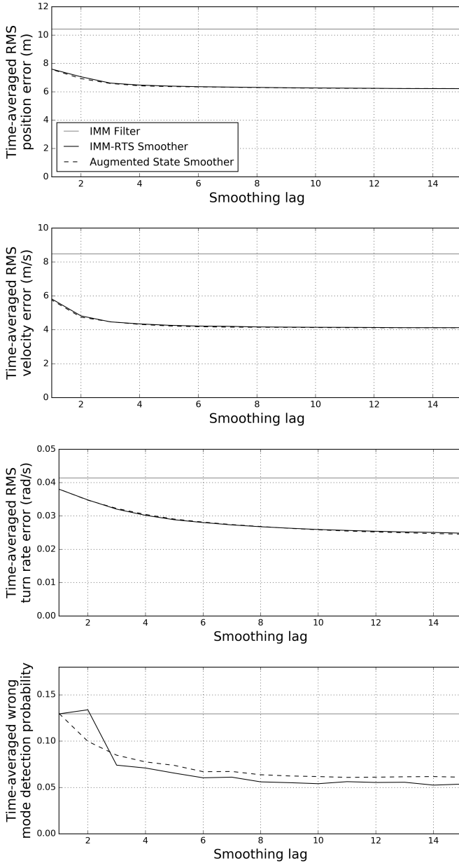
Fig. 4. Comparison of the IMM filter and the fixed-lag smoothers: (from top to bottom) (a) time averaged position RMSE, (b) time averaged velocity RMSE, (c) time averaged turn rate RMSE and (d) time averaged wrong mode detection probability.
