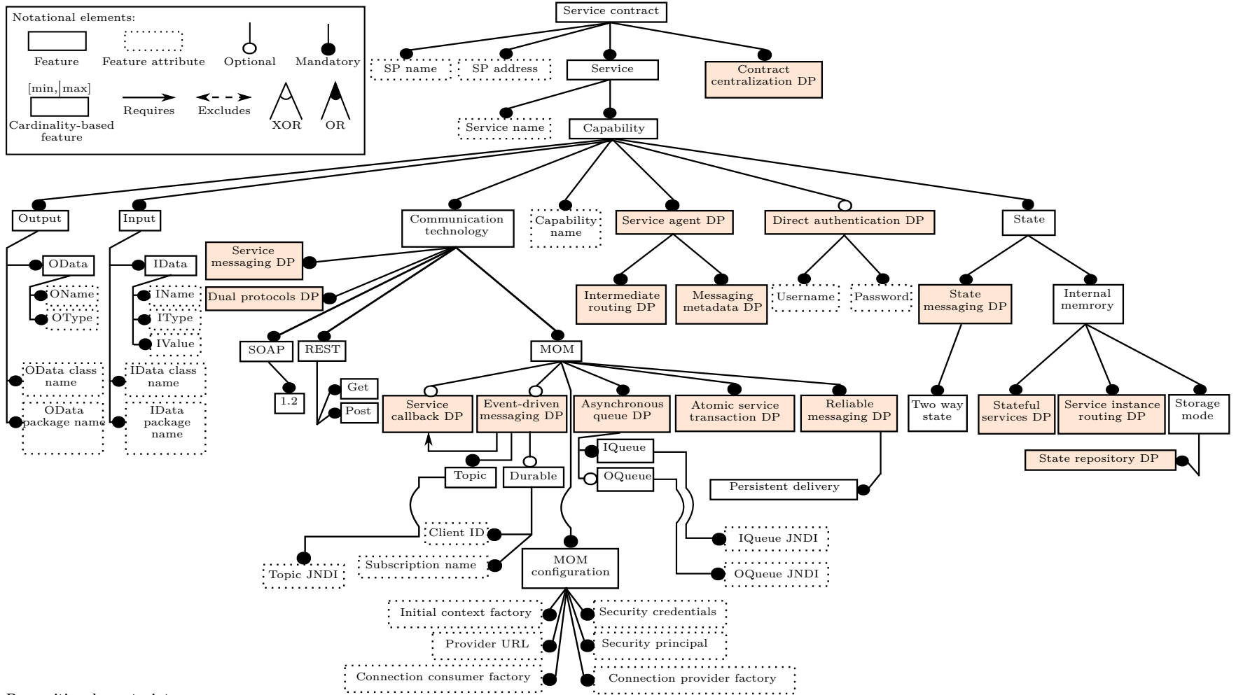
Figure 5: Example of a derived feature model of a service provider FM_{SP_{spec}} from FM_{SP} (design pattern features are colored)
