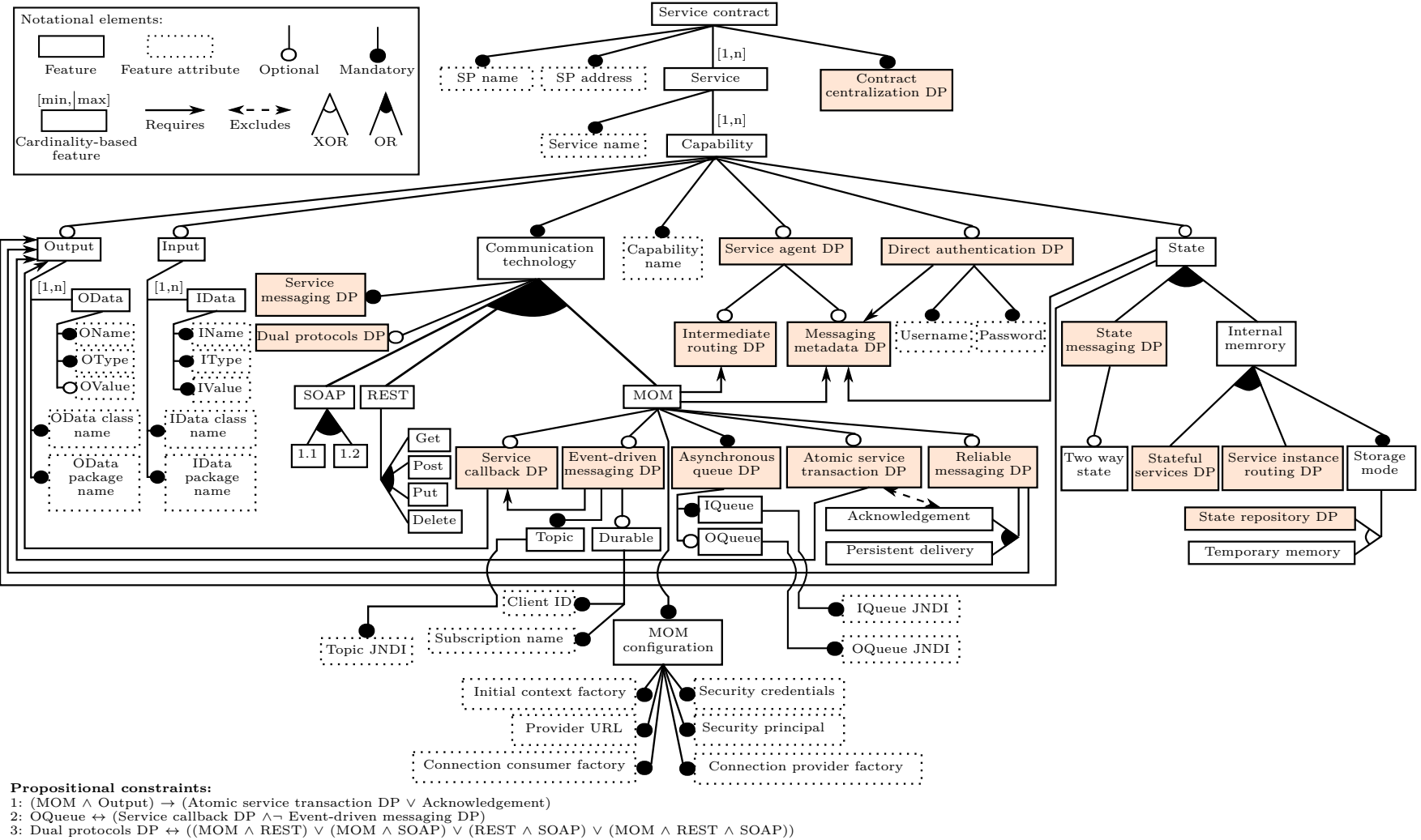
Figure 3: Feature model for the service provider FM_{SP} (design pattern features are colored)
