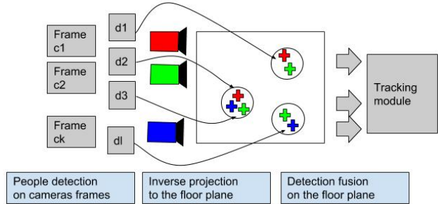
Figure 1: Workflow of our multi-cameras pre-tracking process.
