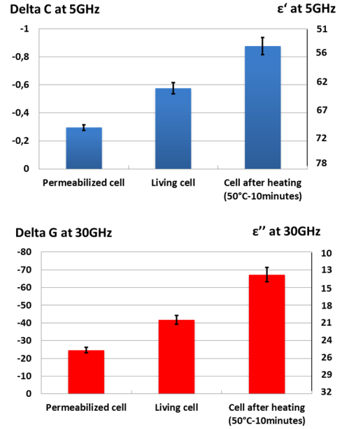
Fig. 4. Average values of the contrasts of different cells states measurements and their dielectric permittivity correspondence obtained with the plots fit of equations (1) and (2).
