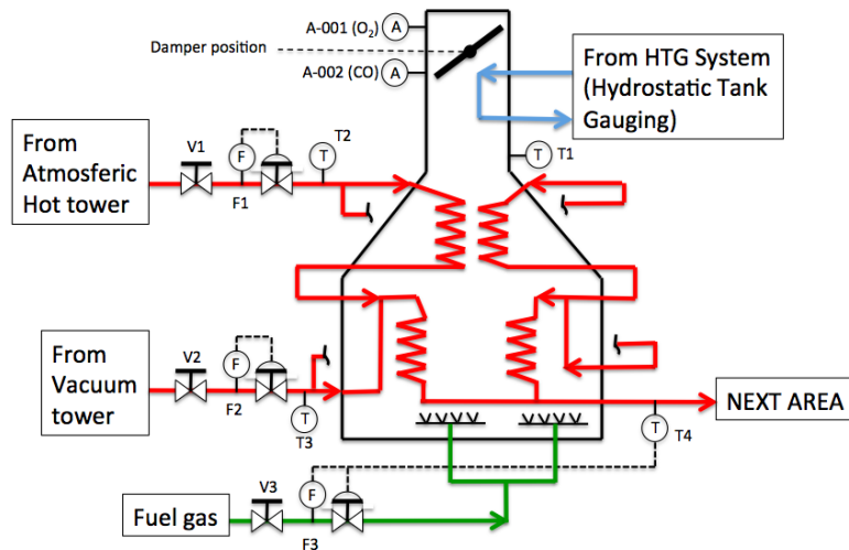
Figure 13: Vacuum oven
