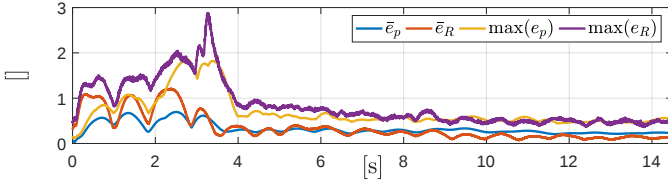
Fig. 9: Exp. 2-1 - Mean of state error function for 23 trials in position (blue) and orientation (red) and maximum state error values over all trials (yellow and purple).
