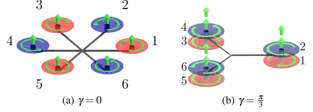
Fig. 2: Two most popular (0,0,\gamma) -hexarotor GTMs: (a) standard star-shaped hexarotor ( \gamma=0 ), (b) Y-shaped hexarotor ( \gamma=\frac{\pi}{3} ).
