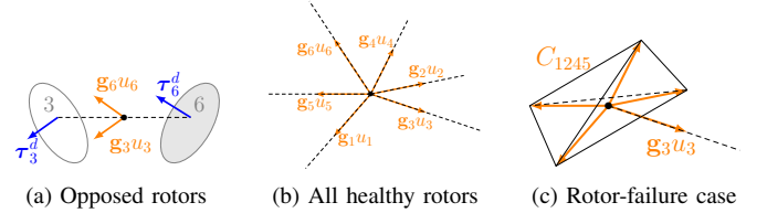
Fig. 4: Composition of the propeller moments for a (0,\beta,0) -hexarotor GTM with any \beta \neq 0 .
