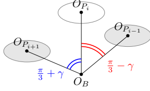
Fig. 1: Position of three consecutive propellers, highlighting the effect of the \gamma angle.
