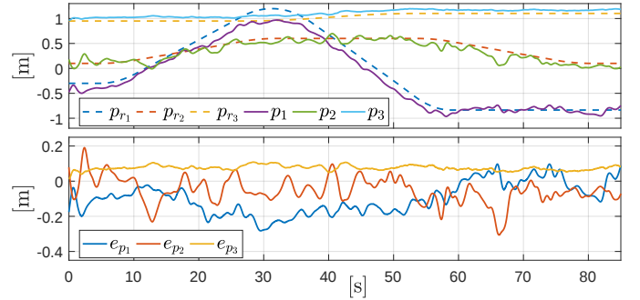
Fig. 11: Exp. 2-3 - Trajectory following of the system with failure.
