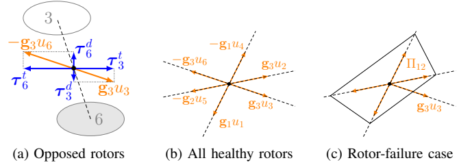
Fig. 3: Composition of the propeller moments for a (\alpha, 0, 0) -hexarotor GTM with any \alpha .
