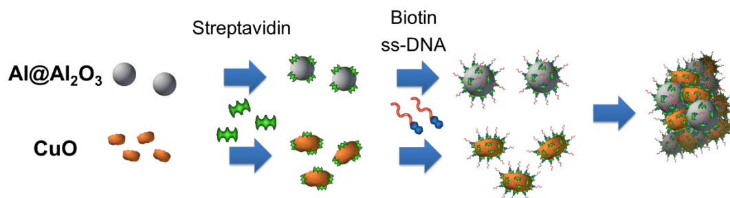
Figure 1. Illustration of the functionalization process developed to enable the DNA-directed self-assembly of \text{Al@Al}_2\text{O}_3 and \text{CuO} nanoparticles.
