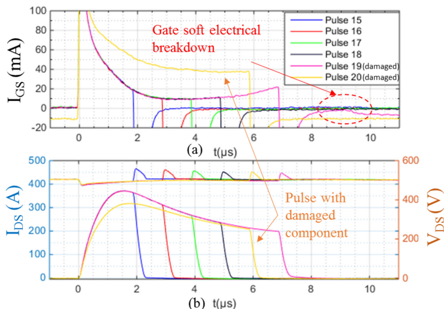
Fig. 2. ST1 device short-circuit waveforms. (a) Evolution of I_G , and (b) V_{DS} , I_D waveforms during the study. Each color represents a SC pulse with an increased on-time. ( V_{DS} = 500\text{V} ; V_{buffer(ON/OFF)} = 18\text{V} / -5\text{V} ; T_{case} = 25^\circ\text{C} ; R_G = 47\Omega ; ST1).
