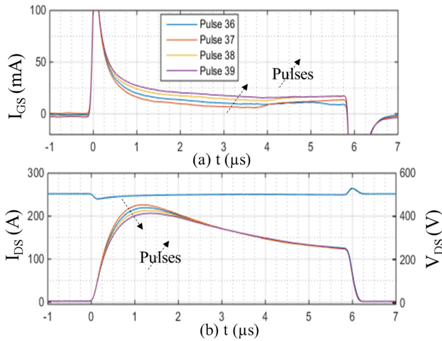
Fig. 3. C1 short-circuit waveforms. (a) Evolution of I_G , (b) V_{DS} and I_D during the study. Each color represents a SC. ( V_{DS}=500V ; V_{buffer(ON/OFF)}=21V/-5V ; T_{case}=25^\circ C ; R_G=100\Omega ; C1).
