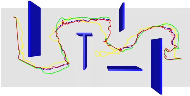
Fig. 5: Comparison of the solution paths for the simple scenario. Paths are shown for one of the four robot. The red line is the raw T-RRT path. The blue one was obtained by T-RRT and NEB smoothing with 10 iterations. The green one was obtained by T-RRT and NEB smoothing with 100 iterations. The yellow one was generated by AT-RRT ( 10^6 iterations).
