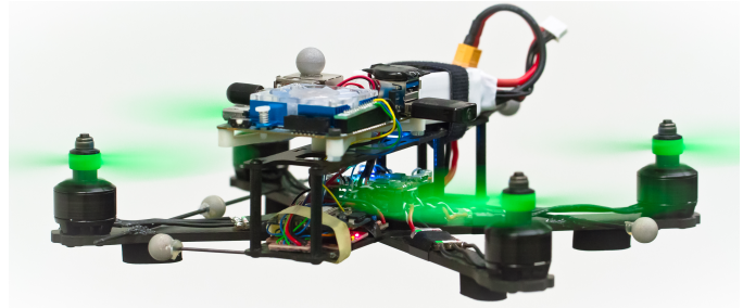
Fig. 1: First-person-view racing inspired quadrotor platform used for the presented experiments.
