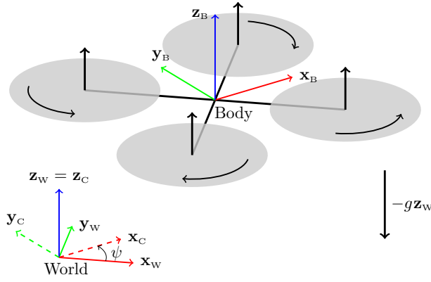
Fig. 2: Schematics of the considered quadrotor model with the used coordinate systems.
