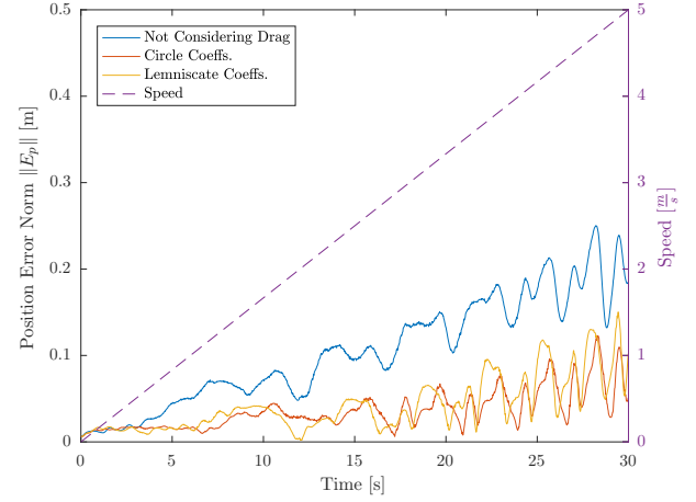
Fig. 6: Position error norm \|E_p\| when ramping the speed on the circle trajectory from 0 \text{ m s}^{-1} up to 5 \text{ m s}^{-1} in 30 s without considering rotor drag (solid blue), with drag coefficients estimated on the circle trajectory (solid red), and with drag coefficients estimated on the lemniscate trajectory (solid yellow). The reference speed on the trajectory is shown in dashed purple.
