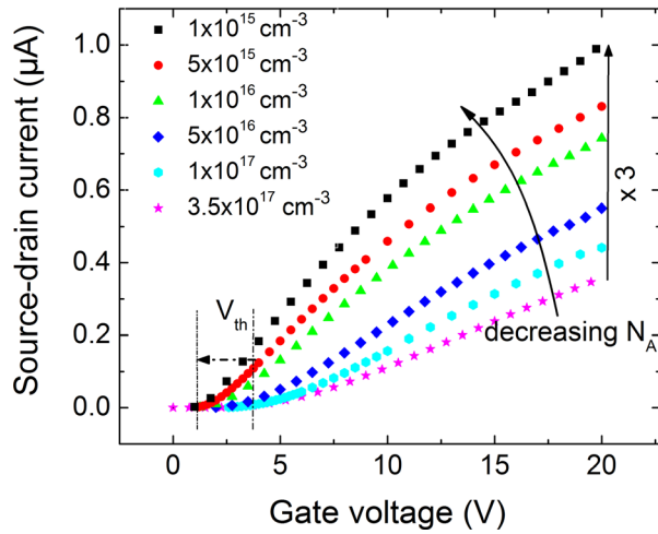
FIG. 1. Drain current as a function of gate voltage for MOSFETs with different acceptor concentrations.
