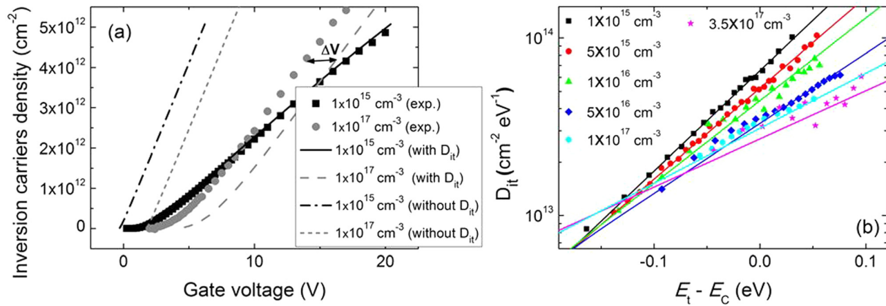
FIG. 3. (a) Experimental (symbols), theoretical (“without D_{it} ”), and calculated (“with D_{it} ”) inversion carriers density as a function gate voltage for devices with N_A of 10^{15} and 10^{17} cm -3 , and curves (b) density of interface states as a function of trap energy for N_A values as specified in the figure.
