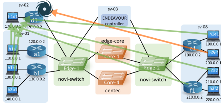
Figure 4: Blackholing topology
