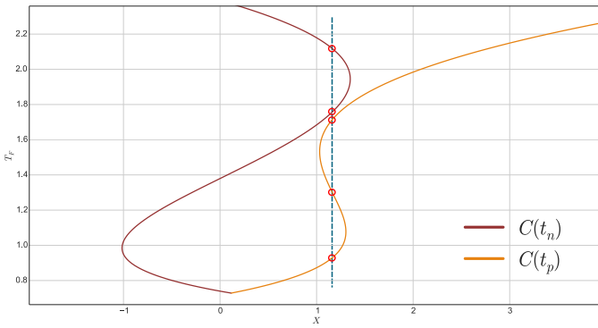
Fig. 10. Curve exhibiting up to 5 solutions when initial and final velocities are shifted. ( J_{min} = -40 , J_{max} = 50 , A_{min} = -55 , A_{max} = 50 , V_{min} = -40 , V_{max} = 70 , a_i = -39.0 ; v_i = 17.205 ; a_f = -39.0 ; v_f = -17.105 ).
