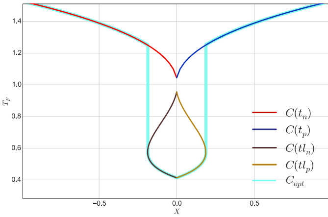
Fig. 9. Shortcut trajectories introduces discontinuities in the time-optimal curve C_{opt} . ( J_{min} = -40 , J_{max} = 40 , A_{min} = -30 , A_{max} = 30 , V_{min} = -30 , V_{max} = 30 , a_i = 20 ; v_i = -4.99 ; a_f = 20 ; v_f = 4.99 ).
