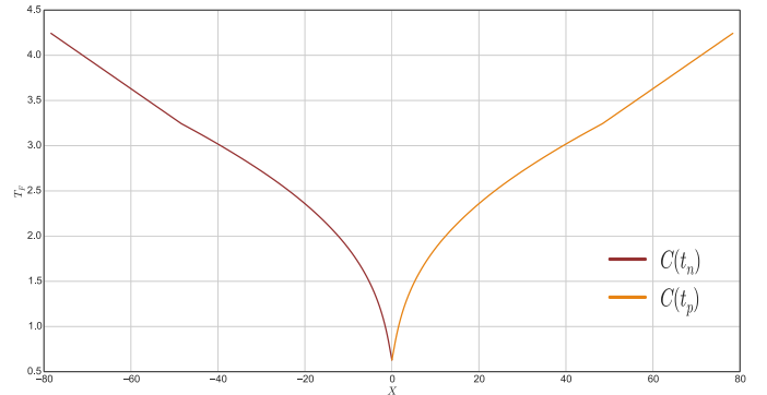
Fig. 6. The optimal ( t_f ) time solutions versus the trajectory length ( x_f ). A trajectory length of zero means the start and end positions are the same. For example the minimum here is associated to the direct trajectory of Fig. 5a, and the null length is explained by the presence of symmetries.
