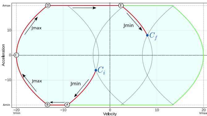
Fig. 2. Phase diagram of a classical seven segments trajectory for a large negative motion. The green area of admissible conditions is limited by the acceleration bounds ( A_{min} , A_{max} ) and the parabolas associated to velocity bounds ( V_{min} , V_{max} ). The jerks J_{min} and J_{max} define four condition parabolas passing through the initial conditions C_i and the final condition C_f . The red curve joins C_f from C_i with the following 7 segments: J_{min} \rightarrow A_{min} \rightarrow J_{max} \rightarrow V_{min} \rightarrow J_{max} \rightarrow A_{max} \rightarrow J_{min} . The segment with saturated speed V_{min} holds on point C .
