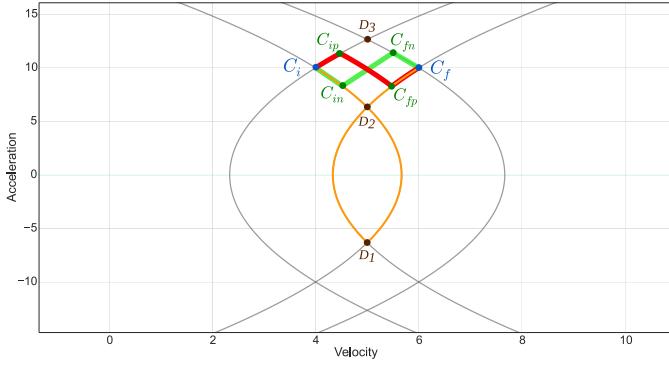
Fig. 4. Limits trajectories in the case where the two parabolas defined by C_i intersect the two parabolas defined by C_f . The main direct trajectory is in orange. The red and green trajectories are two shortcuts trajectories. ( J_{min} = -30 , J_{max} = 30 , A_{min} = -20 , A_{max} = 20 , V_{min} = -20 , V_{max} = 20 , a_i = 10 , v_i = 4 , a_f = 10 , v_f = 6 ).
