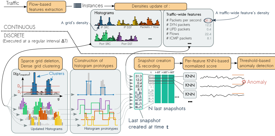
Figure 1: AATAC architecture
