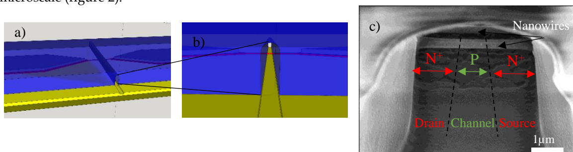
Figure 2. a) and b) schematic views of the Si-nw-ChemFET and the microfluidic channel. c) SEM view of suspended silicon nanowires inside a covered microfluidic channel (tilt 52^\circ ).
