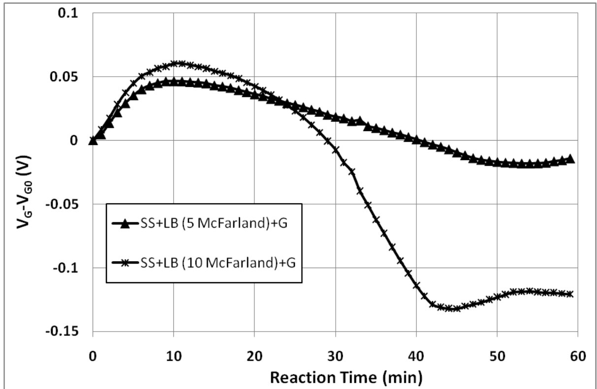
Figure 7: Gate-source voltage V_{GS} variations versus time for two bacteria concentrations (5 and 10 McFarland) with glucose addition ( 20\text{g.L}^{-1} )
