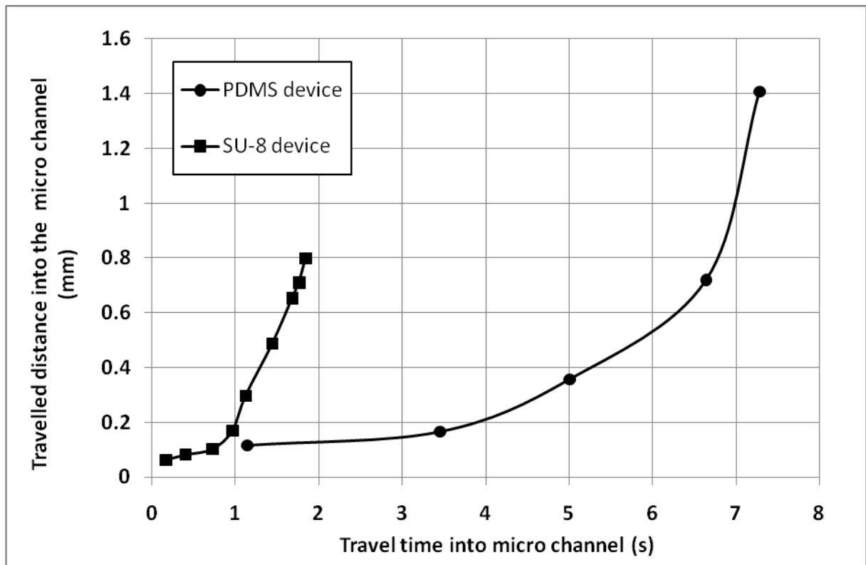
Figure 10: PVA/water mixture (viscosity : 240.2 \times 10^{-3} Pa.s) travelled distance as a function of time, comparison between the PDMS and SU-8 microchannels.
