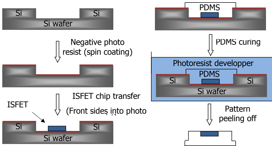
Figure 1: pH-ChemFET chip embedding process in PDMS
