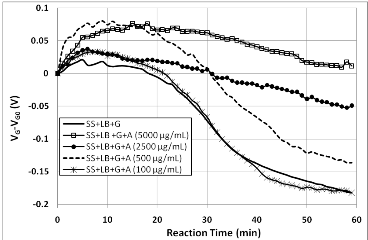
Figure 8: Gate-source voltage V_{GS} variations versus time during glucose assimilation in presence of ampicillin (A) for a Lactobacillus Crispatus strain
