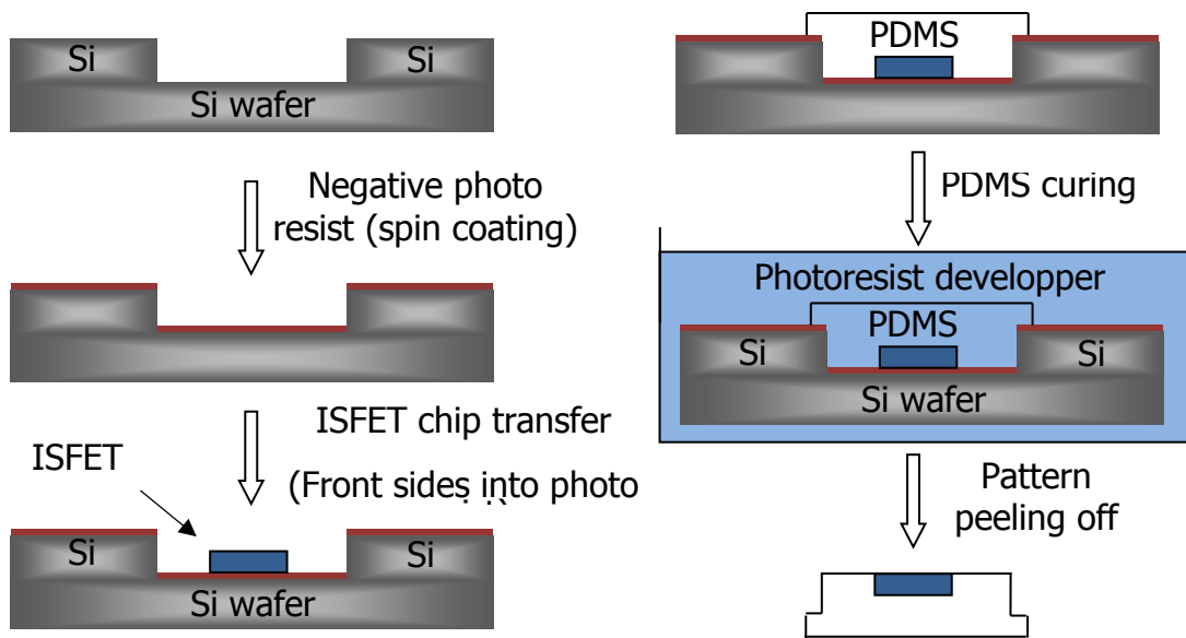
Figure 1: pH-ChemFET chip embedding process in PDMS
