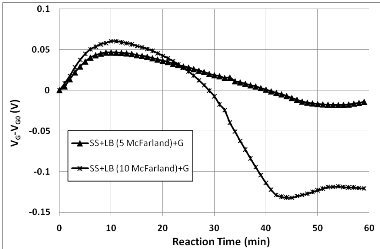
Figure 7: Gate-source voltage V_{GS} variations versus time for two bacteria concentrations (5 and 10 McFarland) with glucose addition ( 20\text{g}\cdot\text{L}^{-1} )
