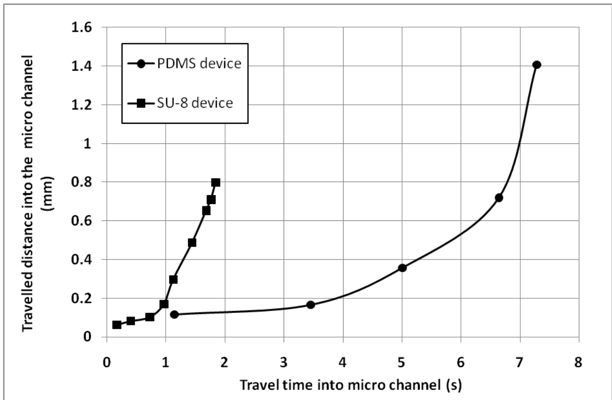
Figure 10: PVA/water mixture (viscosity : 240.2 \times 10^{-3} Pa.s) travelled distance as a function of time, comparison between the PDMS and SU-8 microchannels.
