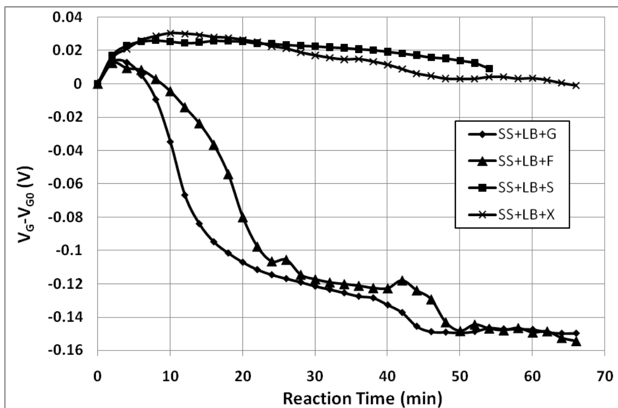
Figure 6: Gate-source voltage V_{GS} variations versus time for different kind of sugar assimilation by a Lactobacillus Crispatus strain – G: Glucose, F: Fructose, S: Sorbitol and X: Xylose (concentration for all sugars 20 \text{ g.L}^{-1} )
