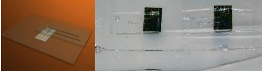
Figure 2: pH-ChemFET chip embedded into PDMS
