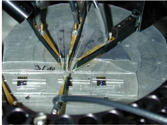
Figure 4: Characterization apparatus
