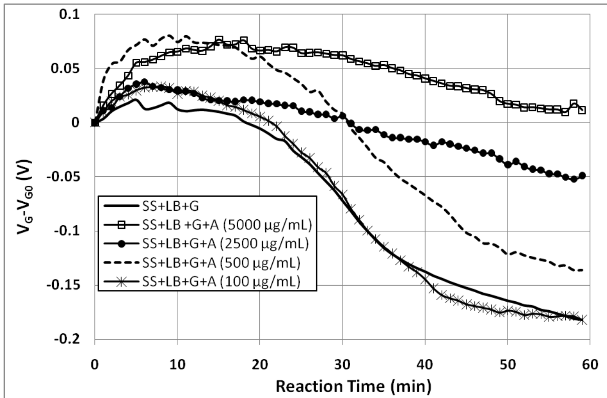
Figure 8: Gate-source voltage V_{GS} variations versus time during glucose assimilation in presence of ampicillin (A) for a Lactobacillus Crispatus strain
