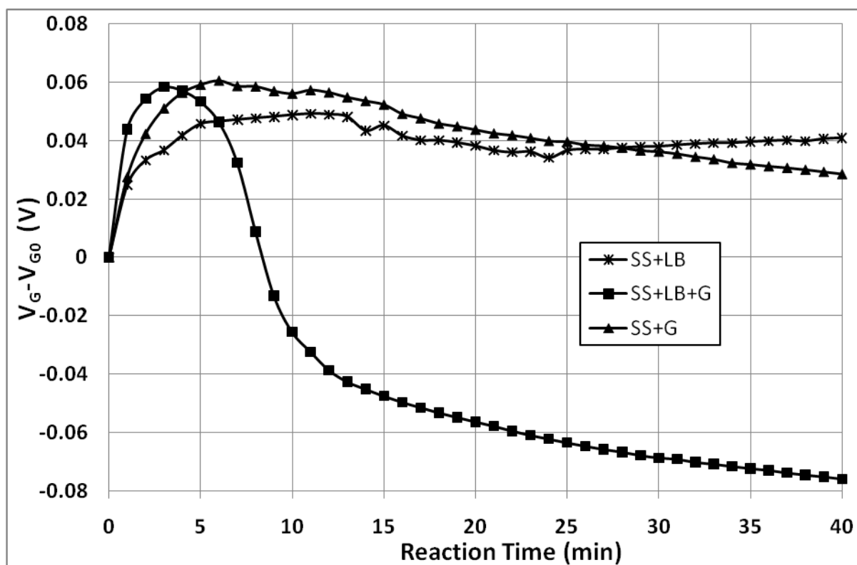
Figure 5: Gate-source voltage V_{GS} variations versus time for various test solutions.
