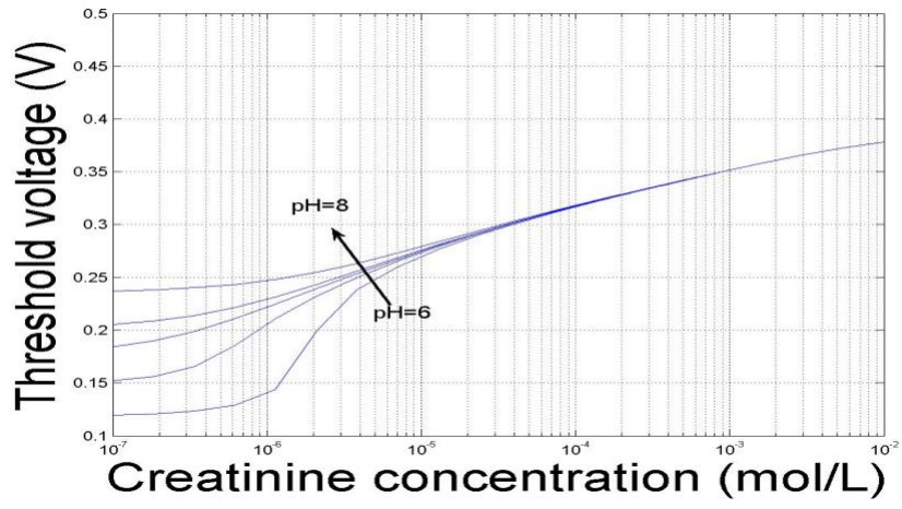
Figure 8: creatinine EnFET responses with solution initial pH value pH 0
