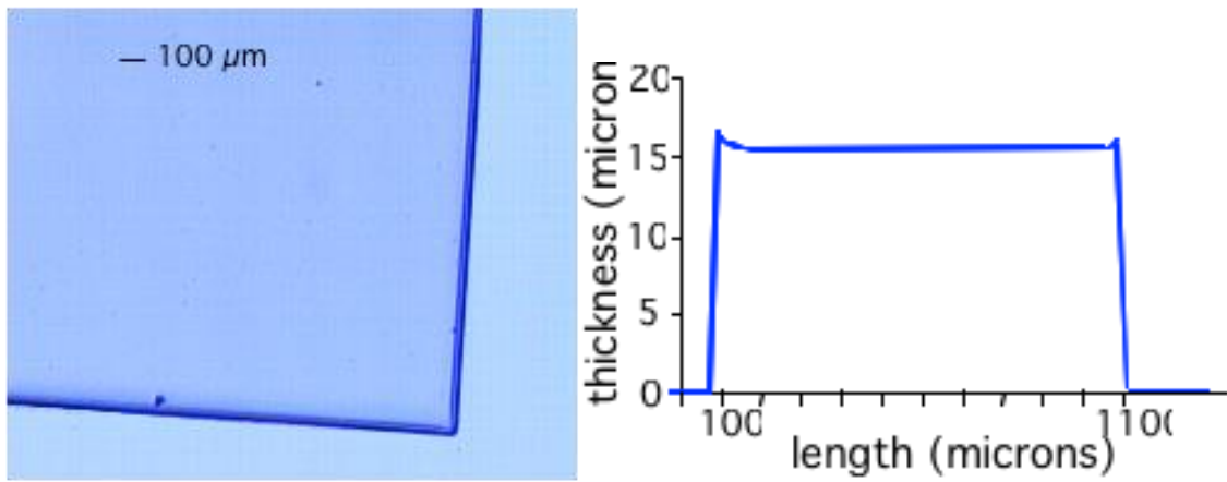
Figure 5: optimized PSX pattern (dimensions: 1000 x 1000 x 15 \mu\text{m}^3 ) picture and profile
