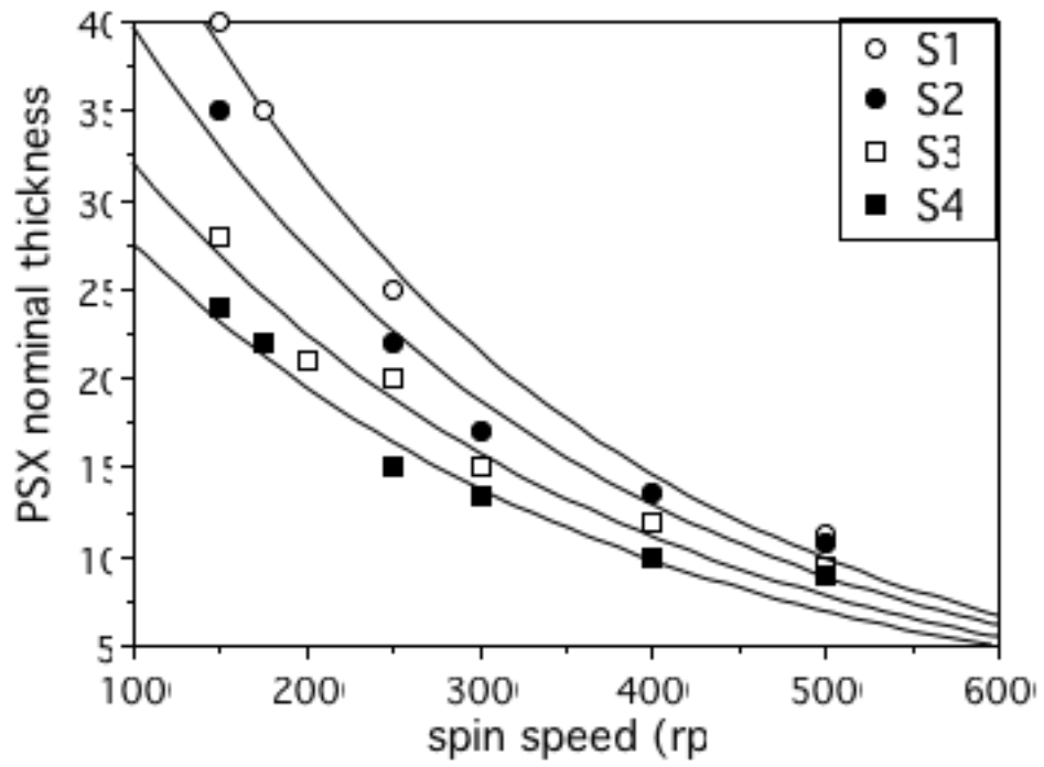
Figure 4: deposited thickness h_{dep} as a function of spin speed \omega for different PSX solutions
