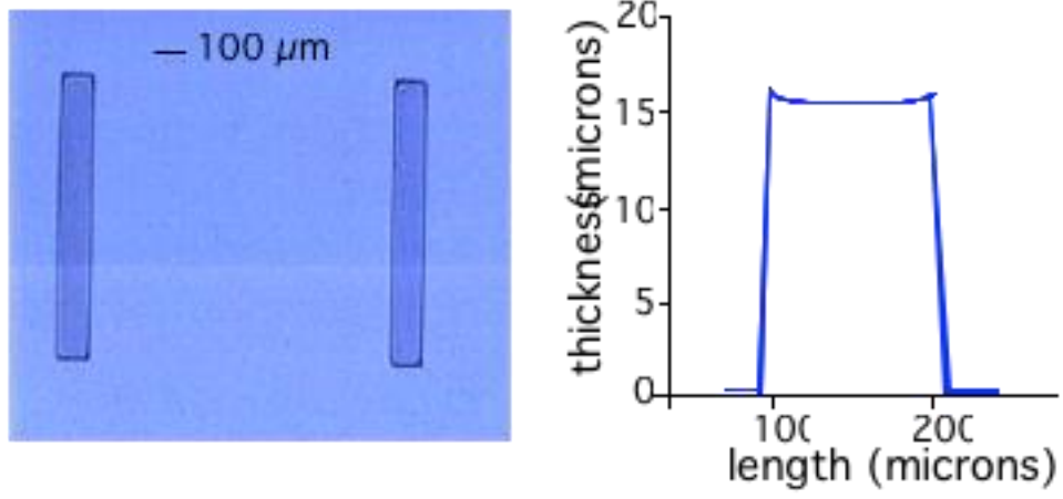
Figure 6: optimized PSX pattern (dimensions: 800 x 100 x 15 μm 3 ) picture and profile
