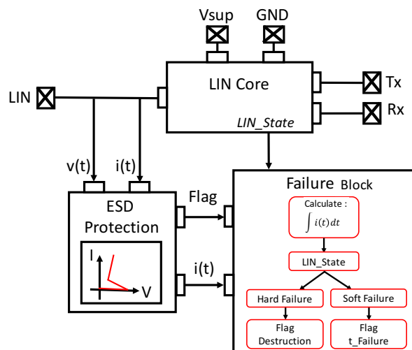
Fig. 1. LIN model behavior for failure investigation
