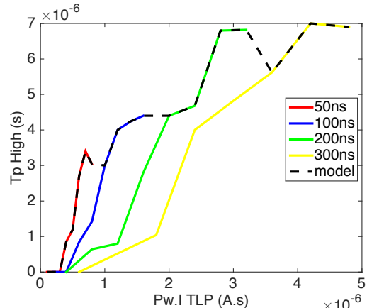
Fig. 11. Failure duration for different pulse widths, state High ( Tp\_High ), related to the product Pw.Itlp (LIN B).
