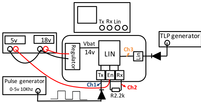
Fig. 3. Schematic of the test bench to charaterize one LIN
