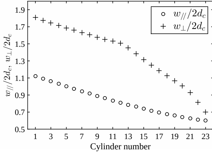
FIGURE 2. Distance between neighbouring cylinders, w_{\parallel} and w_{\perp} (see Figure 1), made dimensionless by dividing by twice the cylinder diameter d_c , plotted as a function of the cylinder number along a given spiral.
