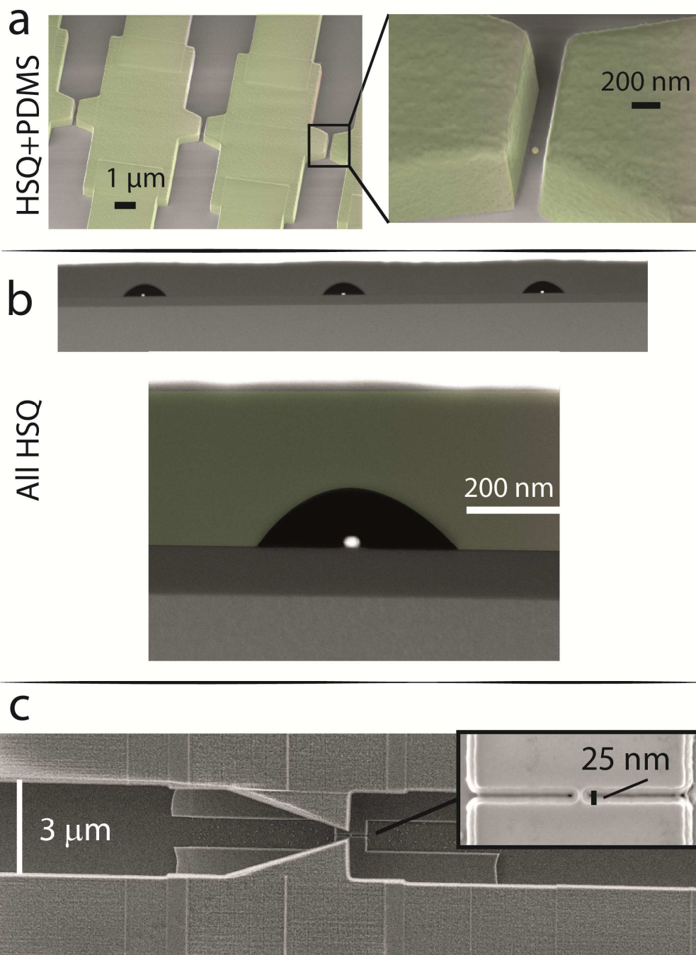
Figure 5. Nanochannels with nanometric alignment precision ability
