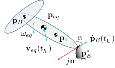
Fig. 2: Notations for the collision model. The large and ‘instantaneous’ reaction force at E is synthesized in the impulse vector j\mathbf{n} .
