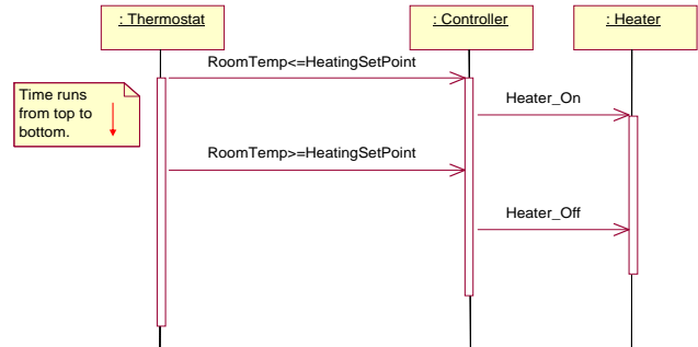
Figure 8. Sequence diagram for building heating mode.
