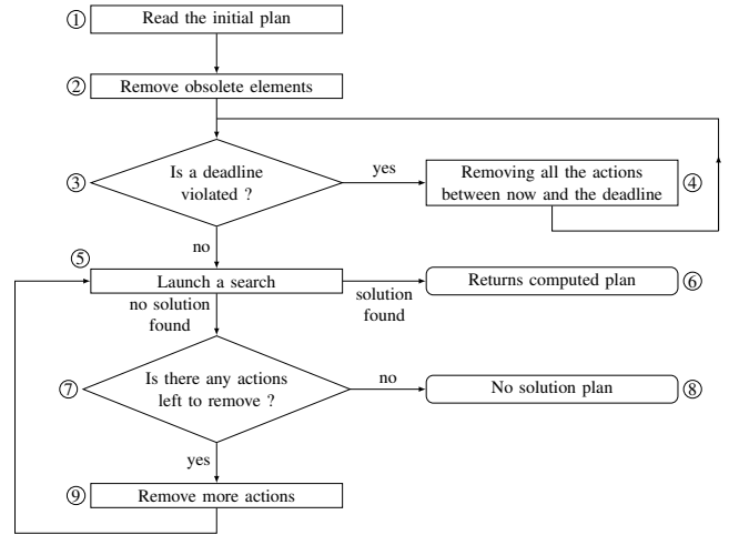
Fig. 2: Iterative Repair Algorithm.
