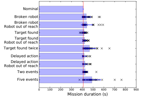
Fig. 3: Duration of the simulated missions. Each cross represents the result of one run. Blue bars represent the average on the 30 runs. The vertical red bar is the average result for the nominal mission.
