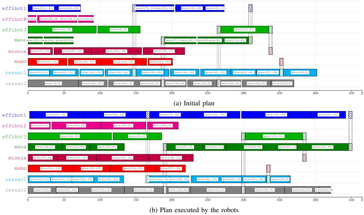
Fig. 6: Temporal representation of plans (x-axis in seconds). Each line represents the plan of one robot. Communications between two robots are represented by the dashed vertical bars. Observation actions are not visible as their duration is null.
