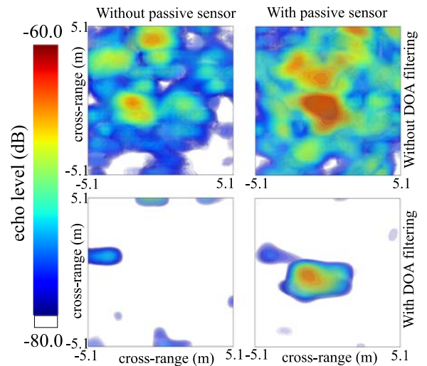
Fig. 10. 2D echo level of the scene at a range R between 57.5 m and 58.5 m with (right) and without (left) the passive humidity sensor. A picture of the experimental setup is shown in Fig. 2(b). Due to the cross-polarization effect, the sensor is detectable at these long distances. A Direction-of-Arrival filter (bottom) removes the undesirable echoes (clutter) and the multi-path generated by the walls of corridor.
