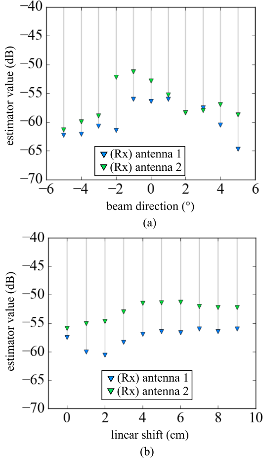
Fig. 11. Humidity estimator e_{Max} computed from the measured electromagnetic echoes of a passive sensor located at 58.0 meters from the radar as a function of: (a) different beam directions with a cylindrical sweeping (solution n°2) and (b) different cross-range positions with a spherical sweeping (solution n°1). The backscattered signal is received by two antenna arrays (Antenna 1 and Antenna 2) of 1x5 patch antennas separated by a distance of 6mm with the gain of 8.6dBi and the beamwidth of 60° and 25° in azimuth and elevation, respectively.
