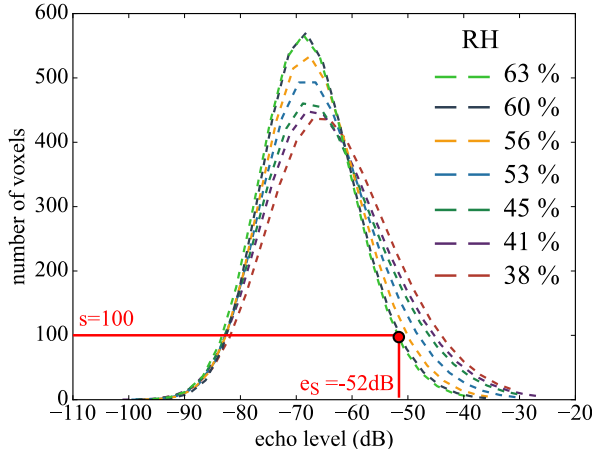
Fig. 4. Measured Gaussian-like distribution of the echo level for various relative humidity using the Van-Atta reflectarray humidity sensor interrogated at 1.3 meters. From this statistical distribution, the estimator e_s is computed for a given number of voxels. As indicated in the figure, for a relative humidity 63% and s=100 voxels, the estimator e_s is found to be of -52dB.
