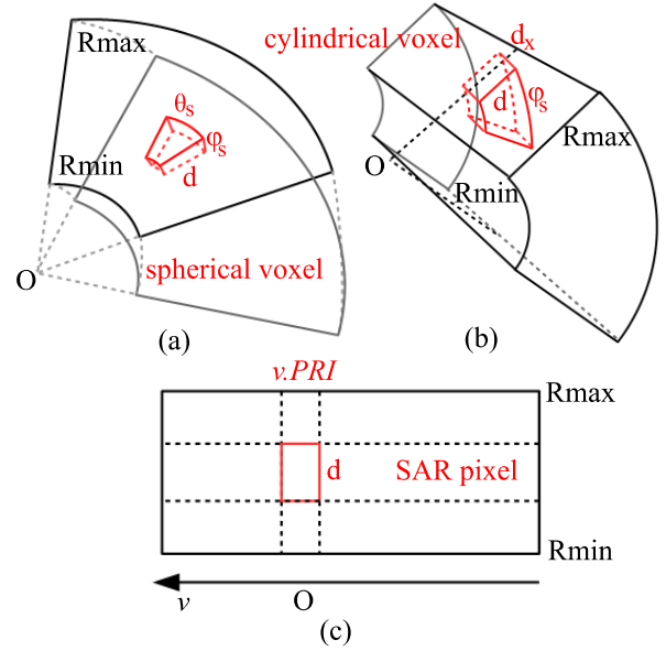
Fig. 3. Voxel generated by: (a) the spherical beam sweeping by a stationary radar, (b) the cylindrical beam sweeping performed by a stationary radar and (c) the SAR-type scanning obtained from the uniform linear motion of the radar with constant velocity v . The point O represents the radar position.
