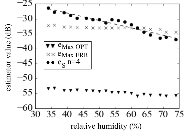
Fig. 7. Statistical estimators e_{MaxOPT} , e_{MaxERR} and e_S(n=4) (see text) as a function of relative humidity using the Van-Atta reflectarray humidity sensor interrogated at 10.0 meters. The estimator e_S(n=4) computed from the sweeping combination solution n^{\circ}4 allows retrieving the sensor echo variation despite the high level of parasitic echoes, embedded in the estimator e_{MaxERR} .
