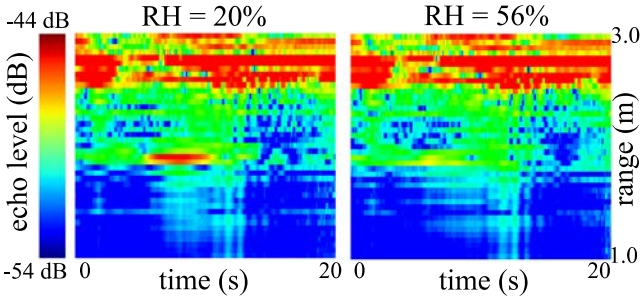
Fig. 9. Two-dimensional display of the electromagnetic echo of Van-Atta reflectarray humidity sensor echo located at 2.1m in front of the radar, for RH=20\% (left) and RH=56\% (right). High echoes observed at 3 meters are due to surrounding clutters.
