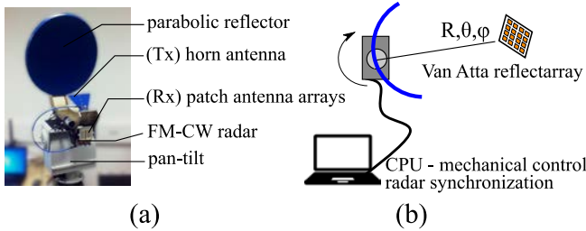
Fig. 1. (a) FM-CW radar interrogation system. Tx and Rx antennas have orthogonal linear polarizations to take advantage of the cross-polarization effect of the relative humidity passive sensor. The mechanical beam scanning in azimuth and elevation is performed using a pan-tilt. [5] (b) The pan-tilt and radar system are synchronized to perform the beam scanning.
