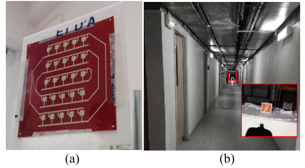
Fig. 2. (a) Kapton-based Van-Atta reflectarray prototype and (b) long range (60 meters) and indoor remote measurement setup of this prototype in a corridor. [5]
