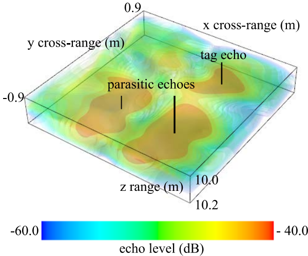
Fig. 6. 3D echo level of the scene at a range R between 10.0 meters and 10.2 meters. It includes the echo response of the tag for RH=37\% as well as parasitic echoes (clutters)
