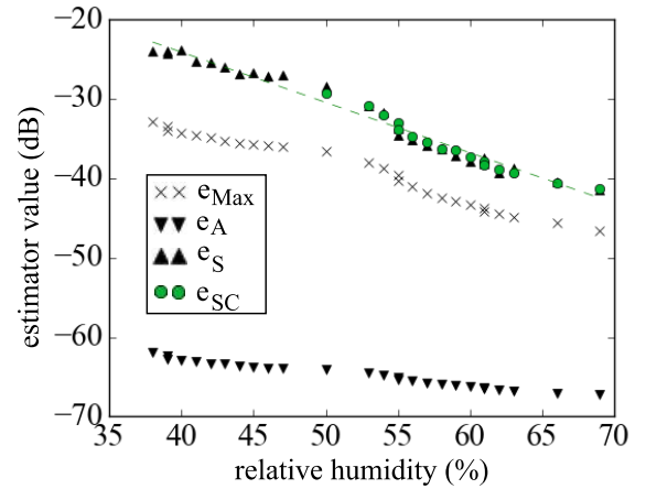
Fig. 5. Statistical estimators e_{Max} , e_A , e_S and e_{SC} (see text) as a function of relative humidity using the Van-Atta reflectarray humidity sensor interrogated at 1.3 meters. A correction (green dots) is applied on the estimator e_S ( s=4 voxels) by taking advantage of the linear behavior of the estimator e_A .
