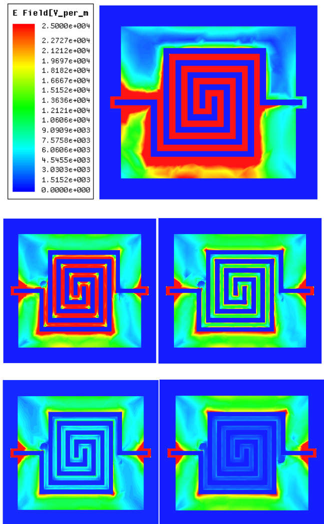
Figure 2: Surface distribution of electric field at 4.5 GHz for four DI water positions.
