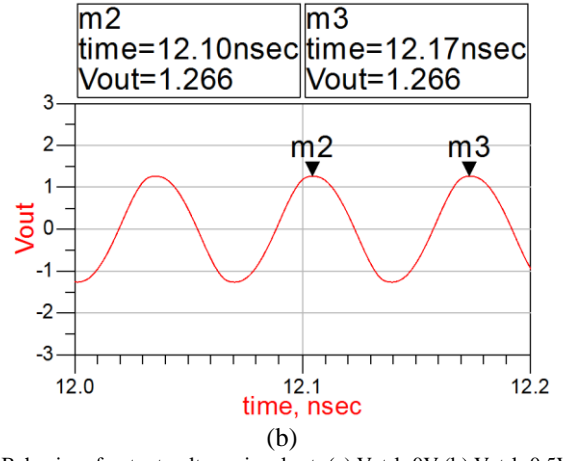
Fig. 6 Behavior of output voltage signals at: (a) V_{ctrl}=0V (b) V_{ctrl}=0.5V .
