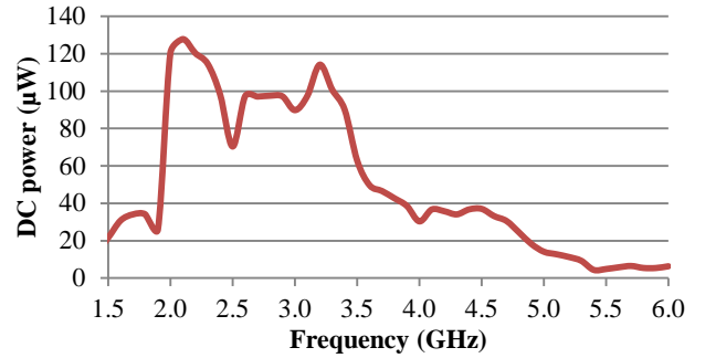
Fig. 6. Measured DC power at the input port of the rectenna load ( 500 \Omega ) as function of frequency. The illuminating E-field varies from E=5.5 V/m to E=10 V/m, depending on the Tx-antenna gain at the considered frequency.
