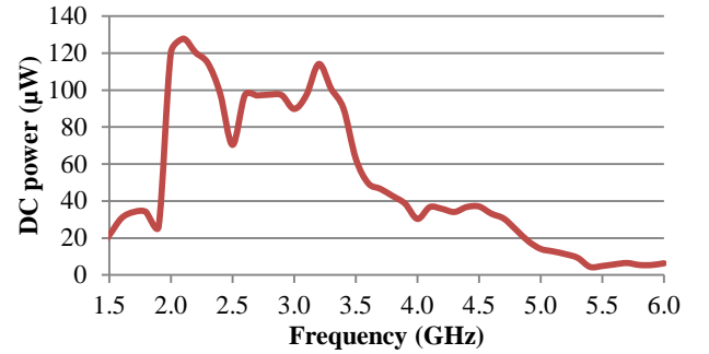
Fig. 6. Measured DC power at the input port of the rectenna load ( 500 \Omega ) as function of frequency. The illuminating E-field varies from E=5.5 \text{ V/m} to E=10 \text{ V/m} , depending on the Tx-antenna gain at the considered frequency.
