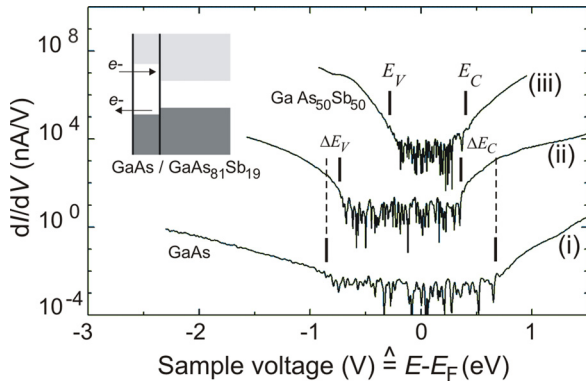
FIG. 3. Tunneling spectra acquired on (i) the pure GaAs top segment and (ii) the shell surrounding the GaAs 81 Sb 19 segment of a GaAs/GaAs 81 Sb 19 /GaAs heterostructure NW, as well as (iii) a GaAs 50 Sb 50 NW. All spectra were acquired at 77 K with tunneling conditions of (i) 1.6 V, 0.8 nA, (ii) 1.6 V, 0.8 nA, and (iii) -1.0 V, 0.5 nA. Spectra (ii) and (iii) have been shifted for clarity. The conduction E_C and valence E_V band edges are indicated by vertical segments, while \Delta E_C and \Delta E_V correspond to the band offsets between GaAs and the GaAs 81 Sb 19 core. Inset: Energy band diagram of the radial GaAs/GaAs 81 Sb 19 heterostructure, the arrows indicating the tunneling of electrons from or into the GaAs 81 Sb 19 core through the GaAs shell.
